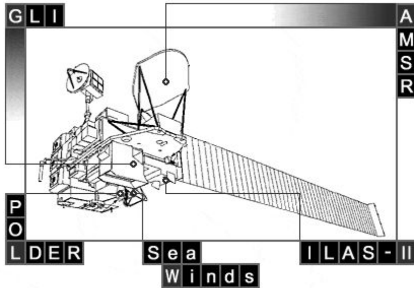
Figure 1.4 ADEOS-II Satellite with Five Instruments
