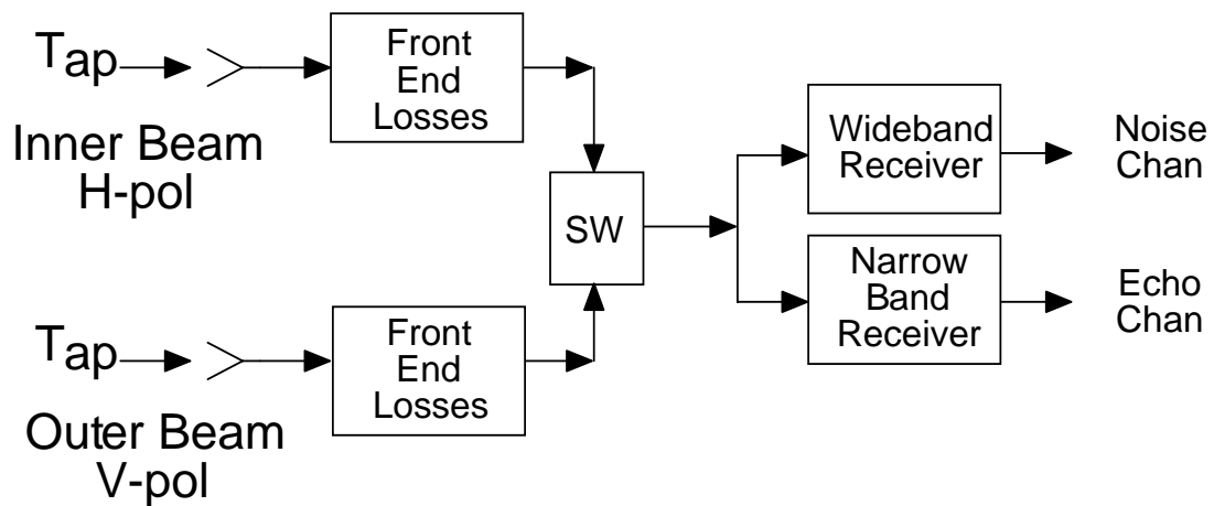
Figure 1.2 SeaWinds Radiometer simplified receiver functional diagram
